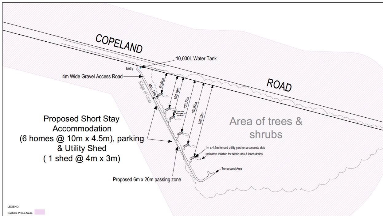
FIGURE 4 – SITE PLAN
